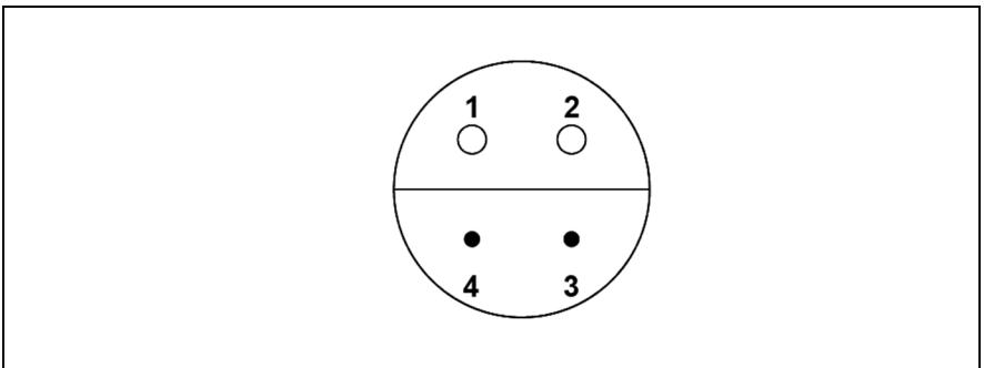
Fig. 7: Connection pin assignment (4-pin)
